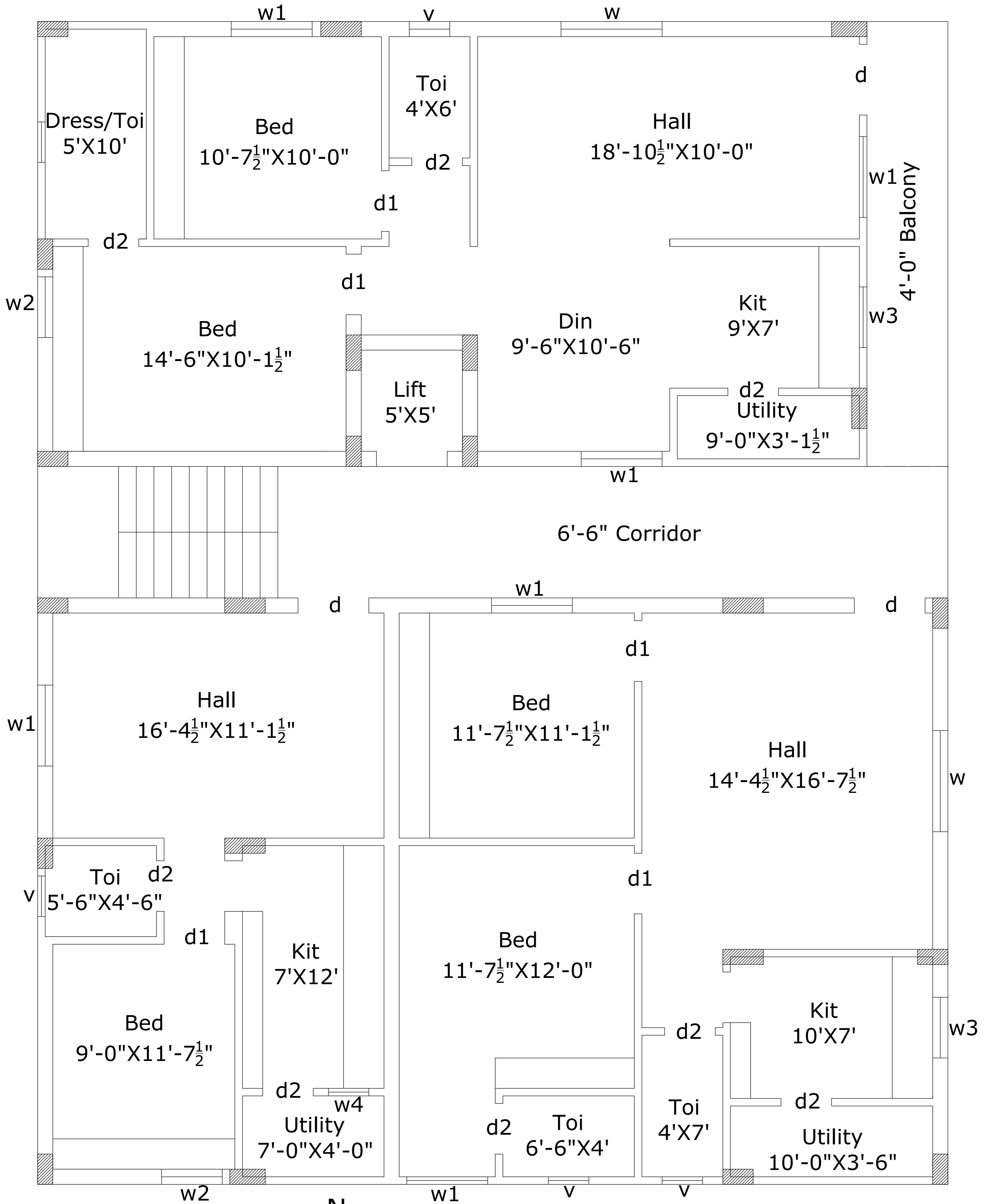
Typical Floor Plan
